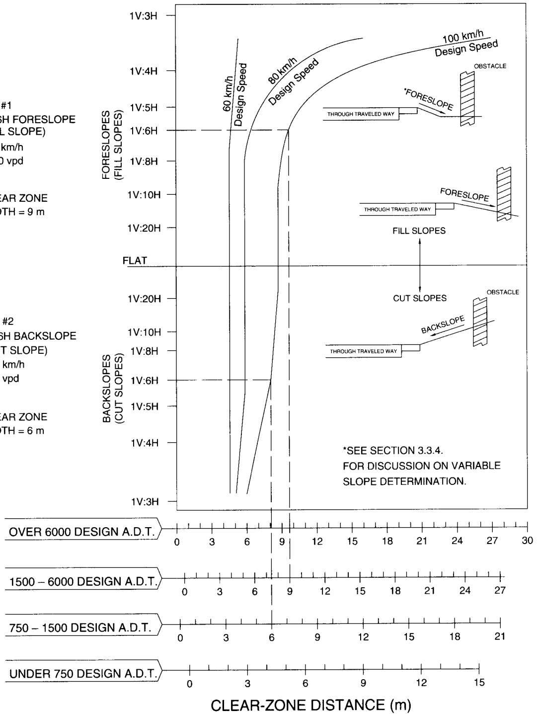
FIGURE 3.1a Clear-zone distance curves [metric units]
