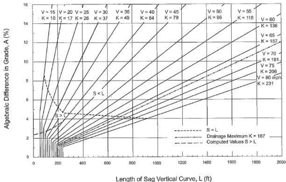
Figure 3-44. Design Controls for Sag Vertical Curves—Open Road Conditions
