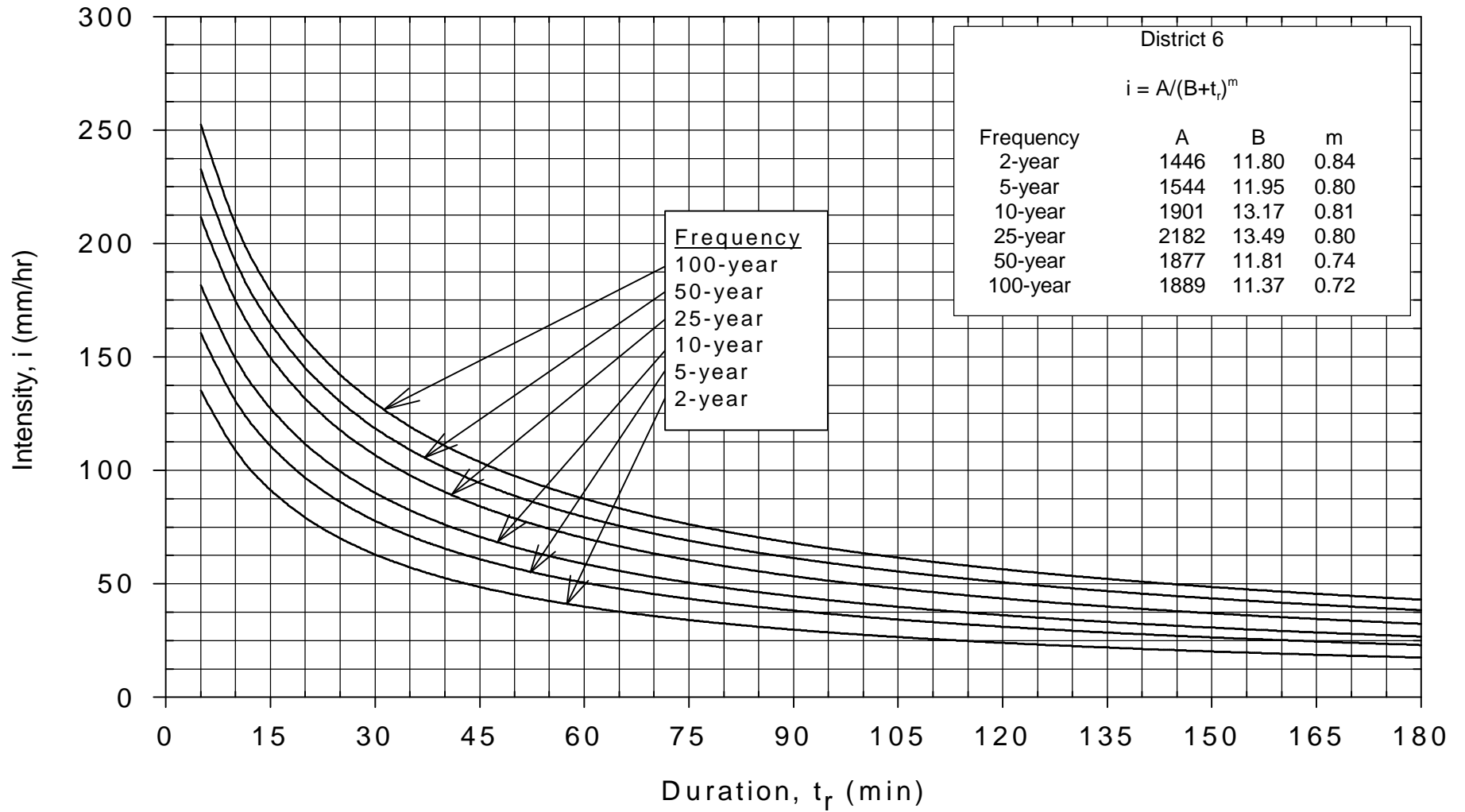
Rainfall Intensity-Duration-Frequency Curves for MoDOT District
