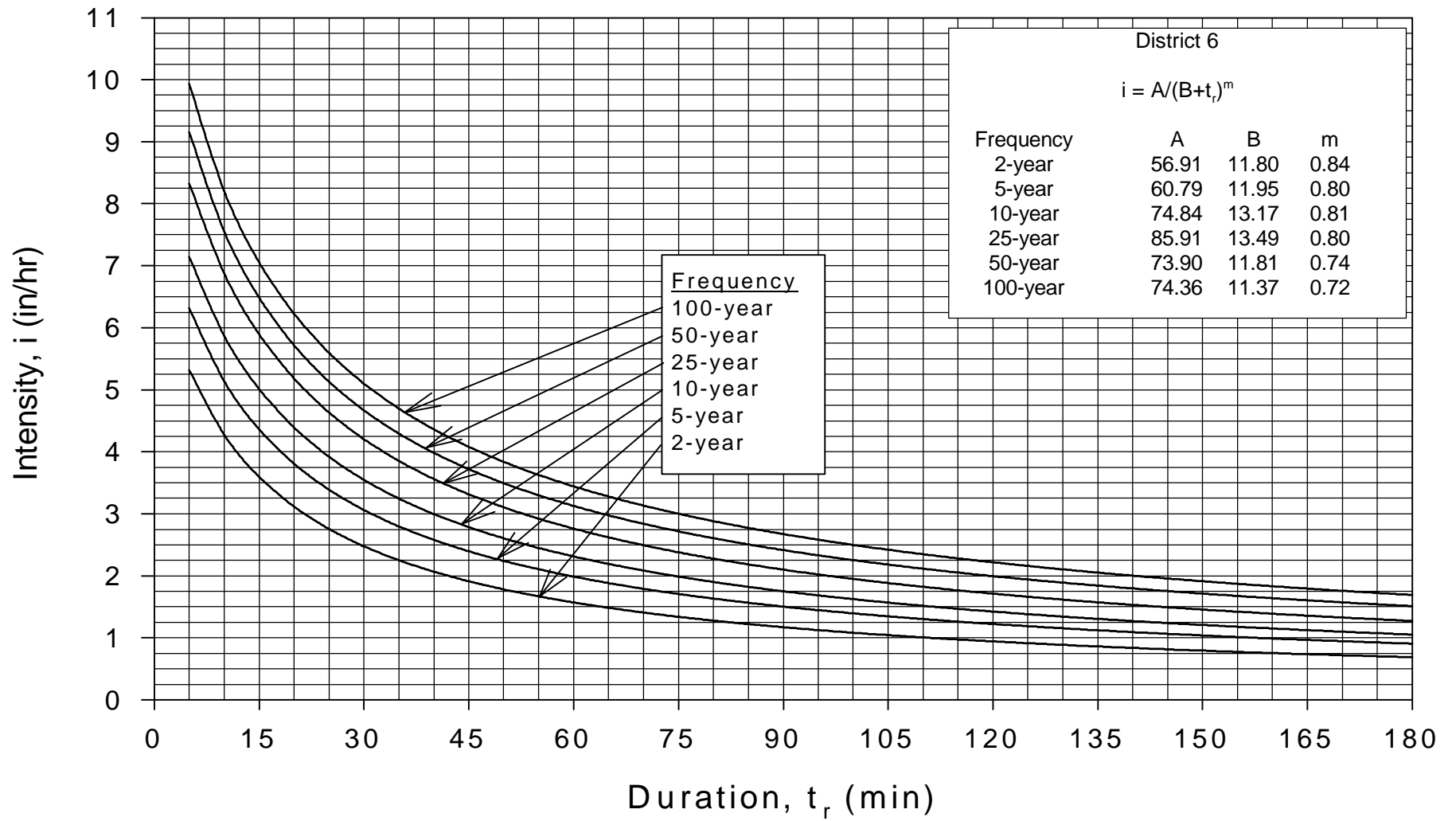
Rainfall Intensity-Duration-Frequency Curves for MoDOT District
