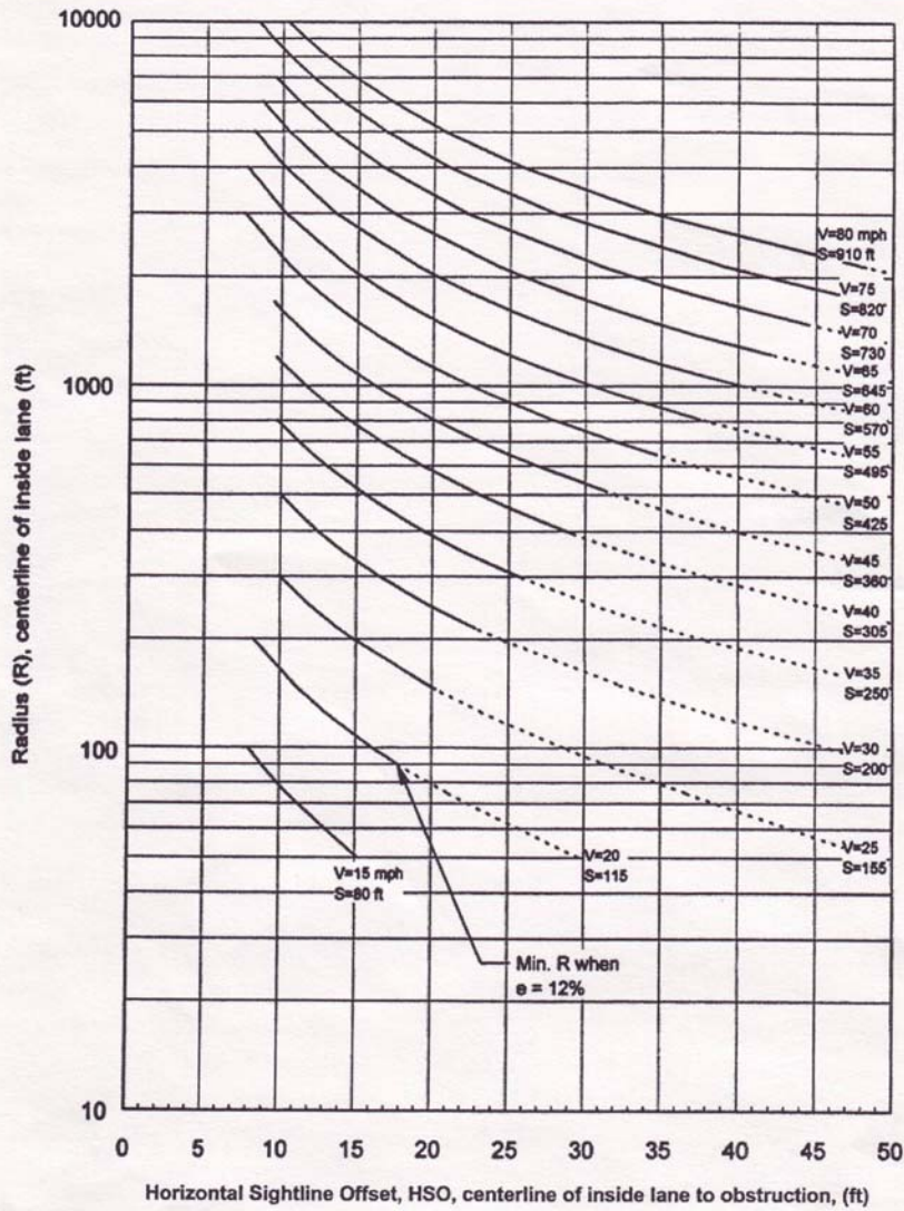
Exhibit 3-53. Design Controls for Stopping Sight Distance on Horizontal Curves (Continued)
