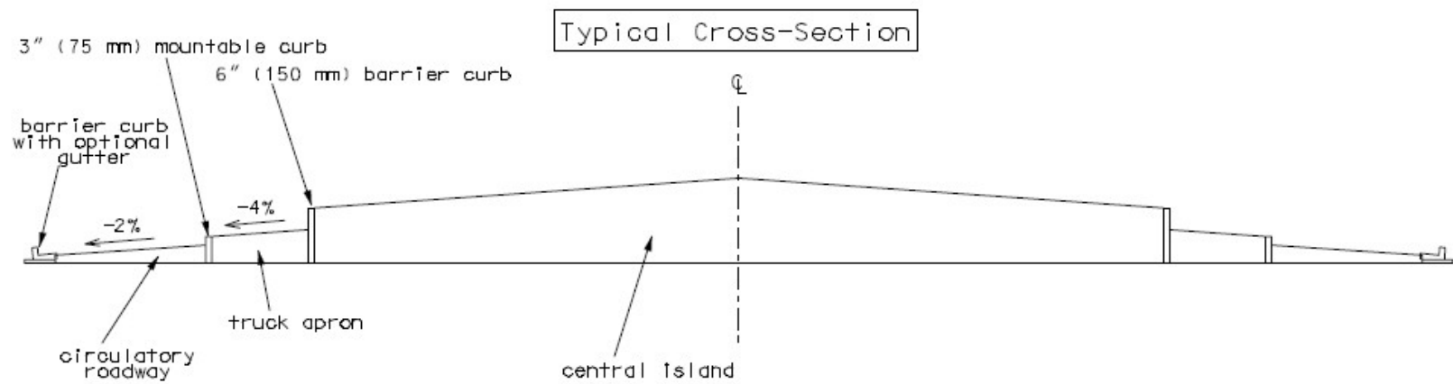
Leg Separation and Typical Cross-Section
