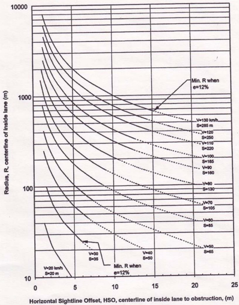
Exhibit 3-53. Design Controls for Stopping Sight Distance on Horizontal Curves
