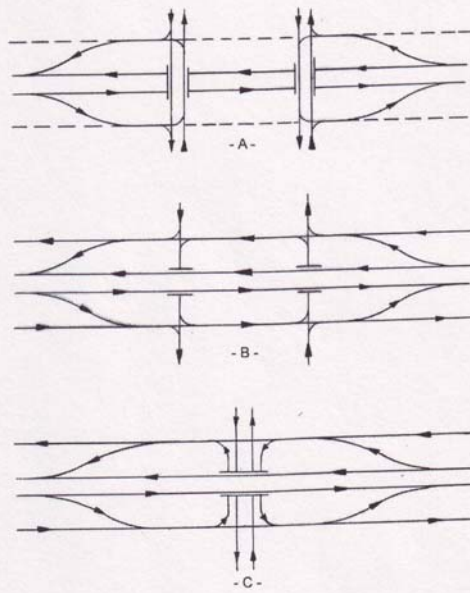
Exhibit 10-17. Diamond Interchange Arrangements to Reduce Traffic Conflicts
