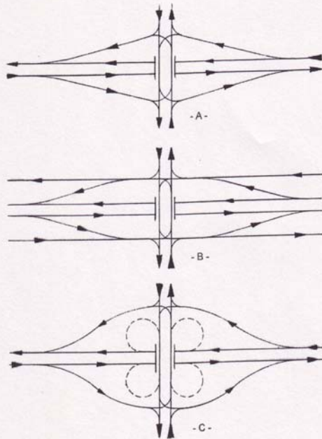
Exhibit 10-16. Diamond Interchanges, Conventional Arrangements
