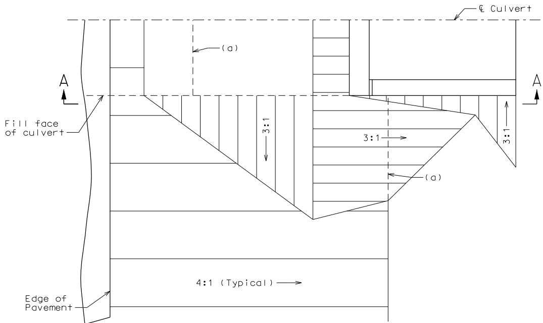
PART PLAN
