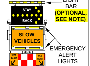
SHOULDER ADVANCED WARNING TRUCK (4) (5) (BACK OF TRUCK)
