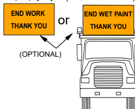
(4)(5) SHOULDER ADVANCED WARNING TRUCK (FRONT OF TRUCK)
