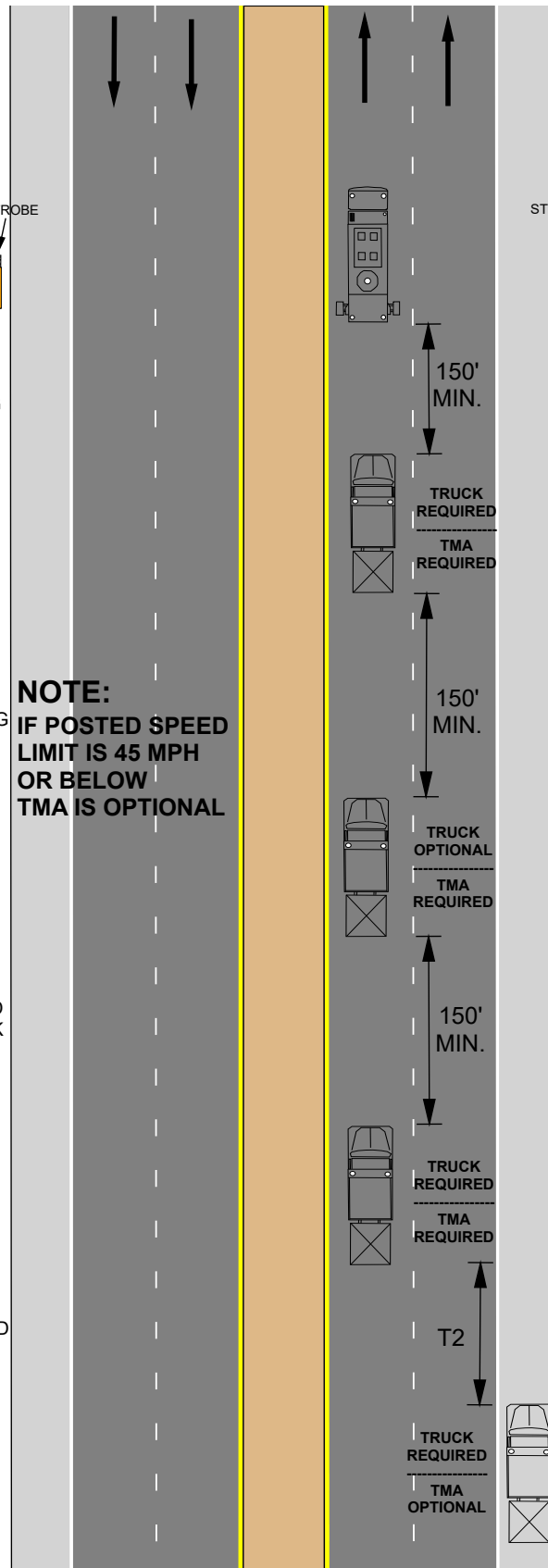
STRIPER (FRONT OF TRUCK)
