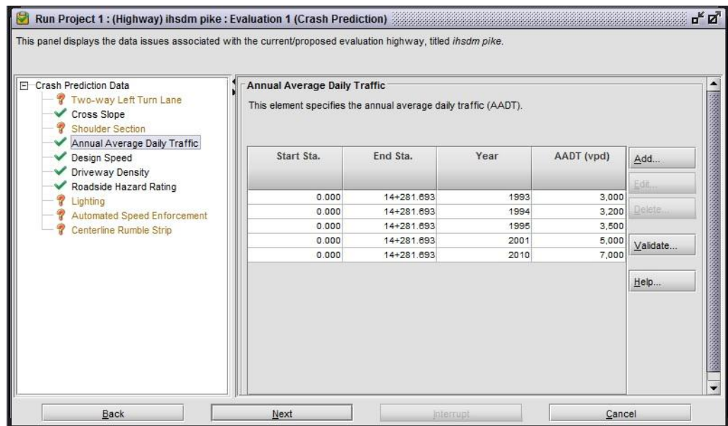
Figure 4.9 Sample input screen from IHSDM software (FHWA).
