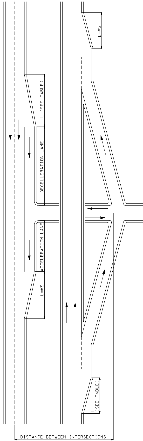
Type 5 Median Opening Partial Grade Separated Intersection
